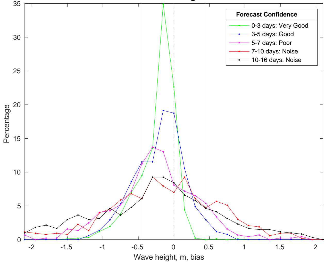
NDBC 41013 vs GFS Waves Bias Histogram: 08-Mar-2025
