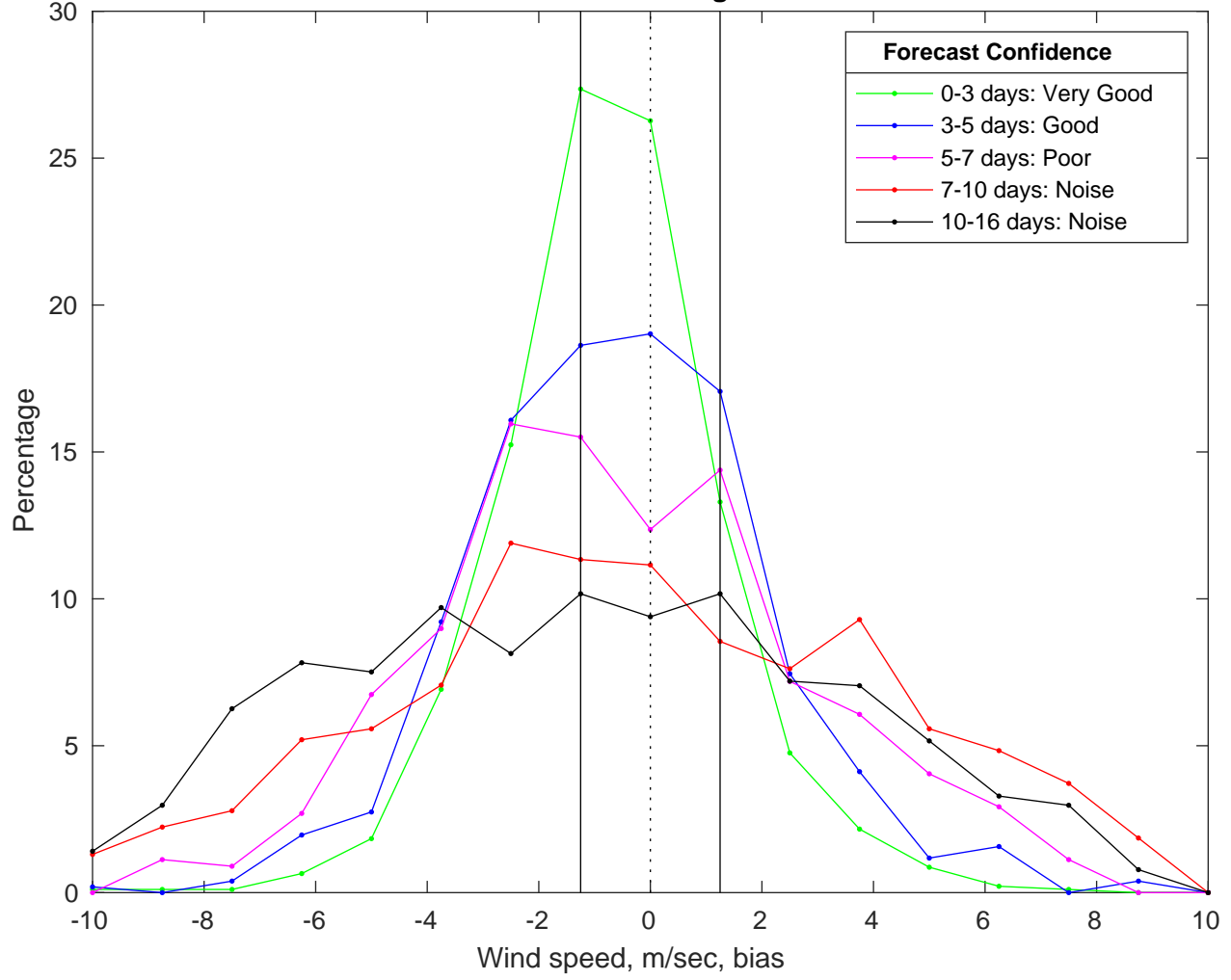
NDBC 41013 vs GFS Winds Bias Histogram: 08-Mar-2025
