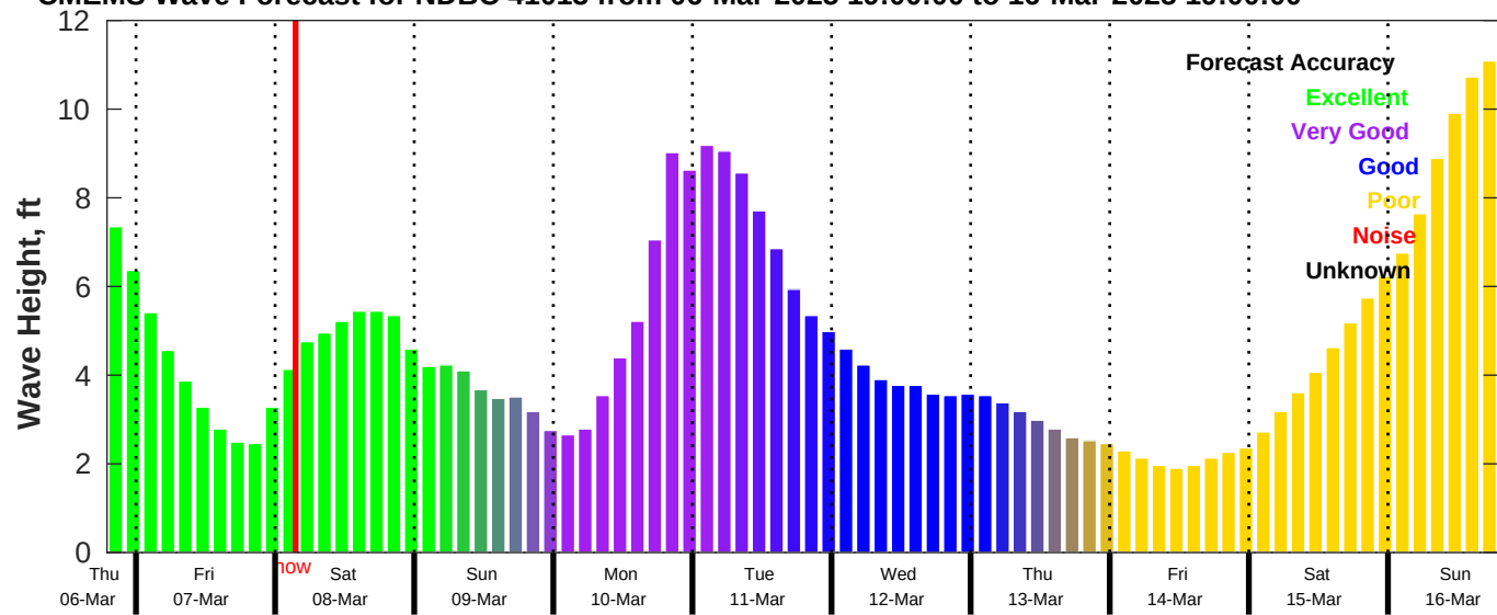
CMEMS Wave Forecast for NDBC 41013 from 06-Mar-2025 19:00:00 to 16-Mar-2025 19:00:00
