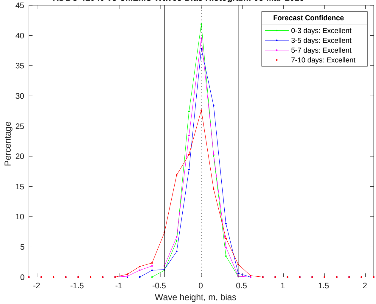
NDBC 41040 vs CMEMS Waves Bias Histogram: 08-Mar-2025
