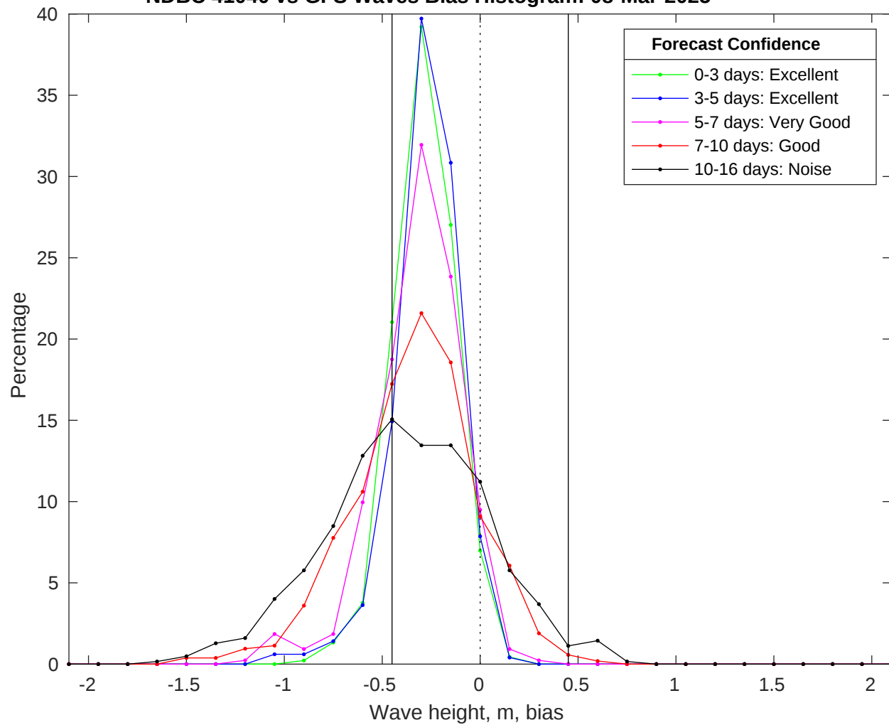
NDBC 41040 vs GFS Waves Bias Histogram: 08-Mar-2025
