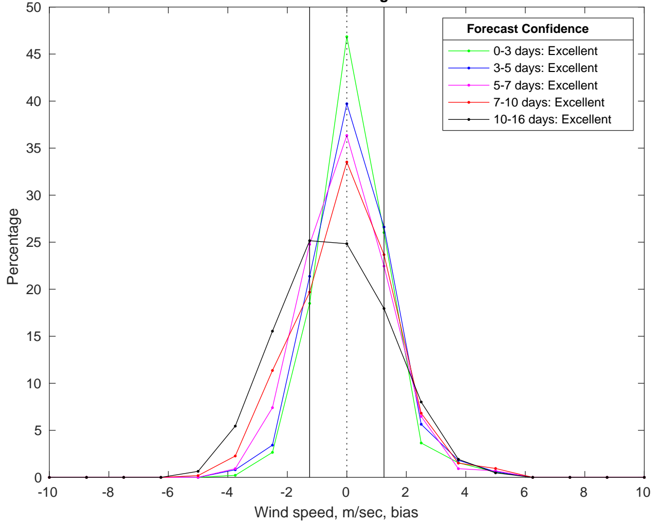
NDBC 41040 vs GFS Winds Bias Histogram: 08-Mar-2025
