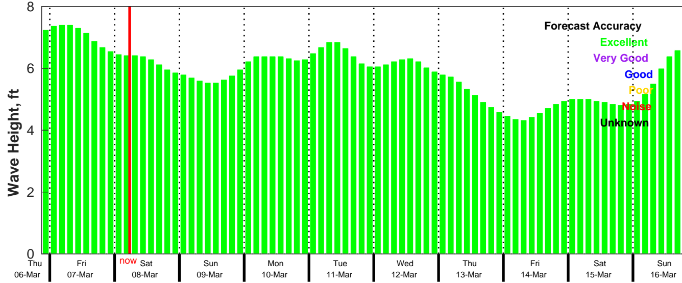
CMEMS Wave Forecast for NDBC 41040 from 06-Mar-2025 21:00:00 to 16-Mar-2025 21:00:00
