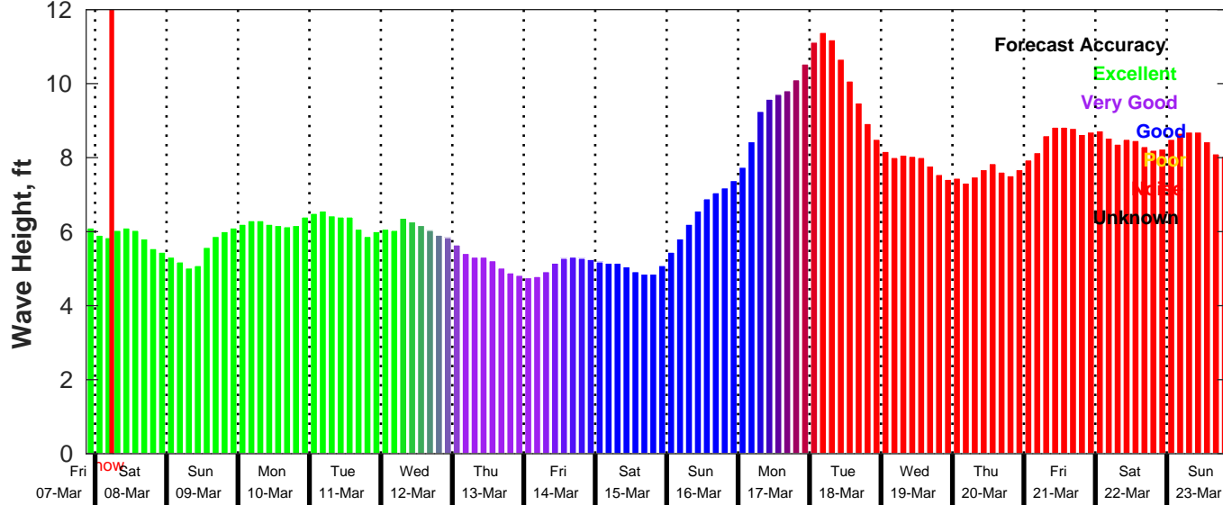
GFS Wave Forecast for NDBC 41040 from 07-Mar-2025 21:00:00 to 23-Mar-2025 21:00:00
