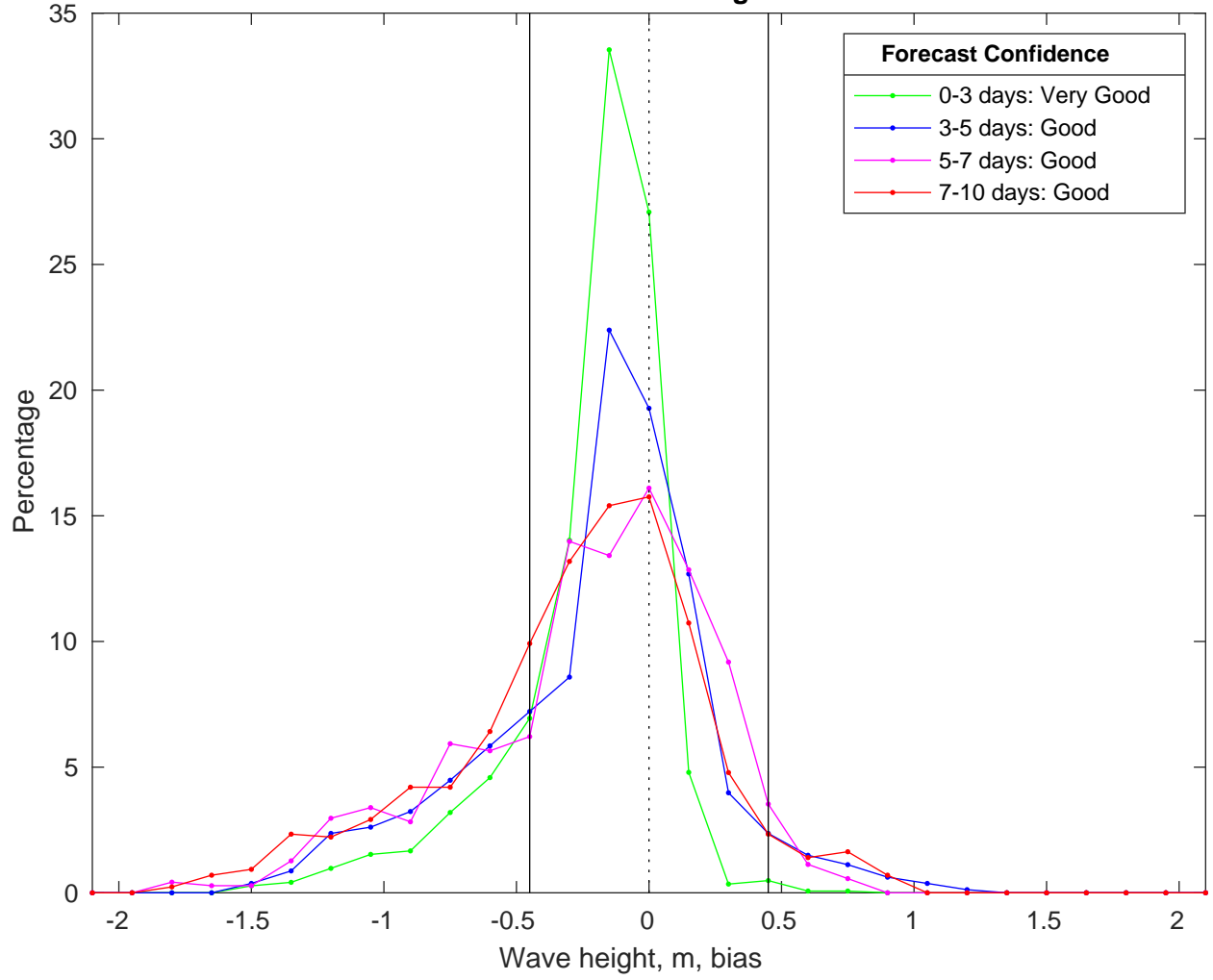
NDBC 42019 vs CMEMS Waves Bias Histogram: 08-Mar-2025
