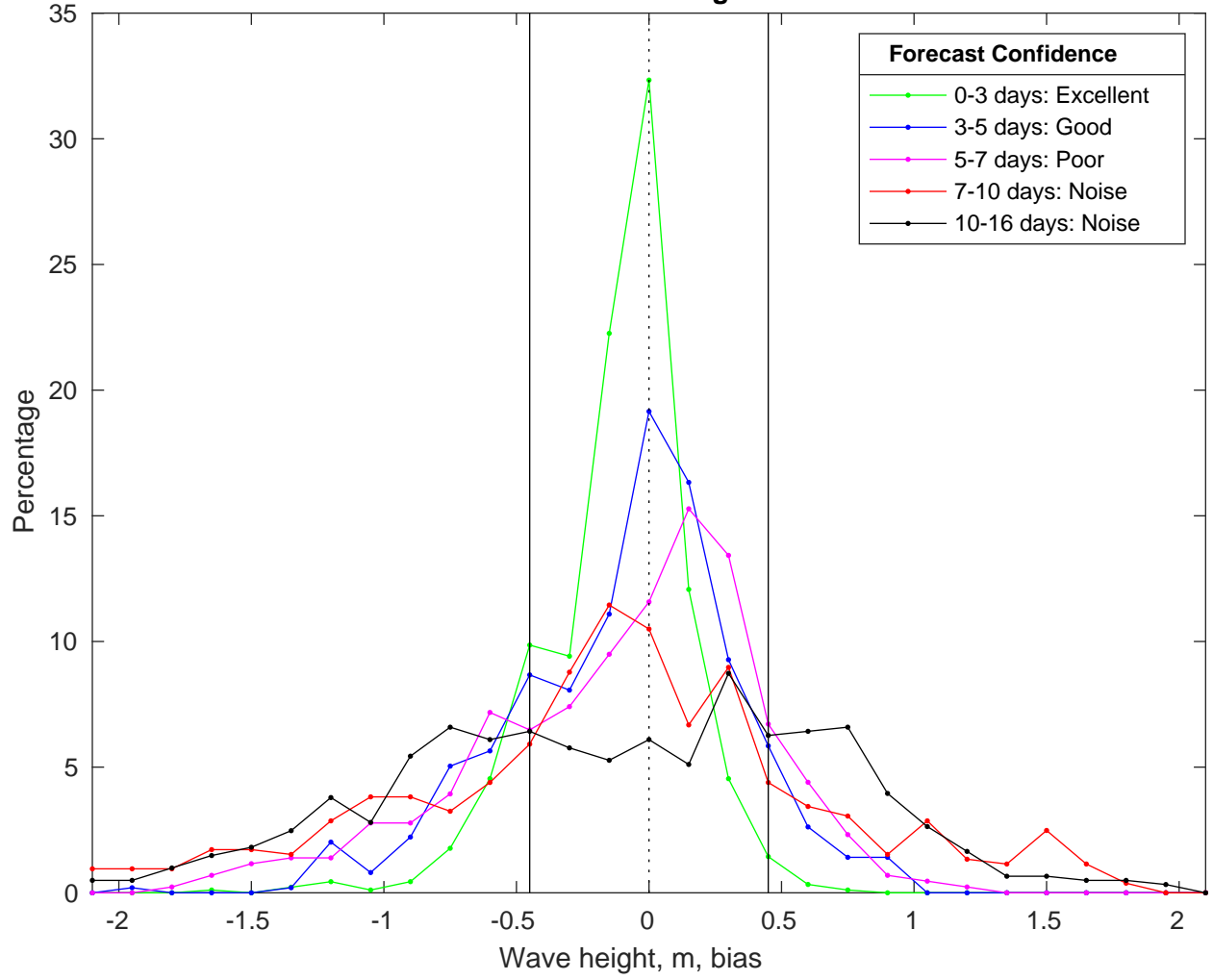
NDBC 42019 vs GFS Waves Bias Histogram: 08-Mar-2025
