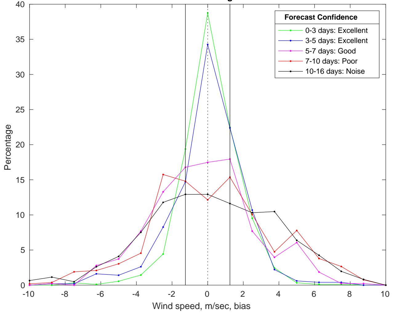
NDBC 42019 vs GFS Winds Bias Histogram: 08-Mar-2025
