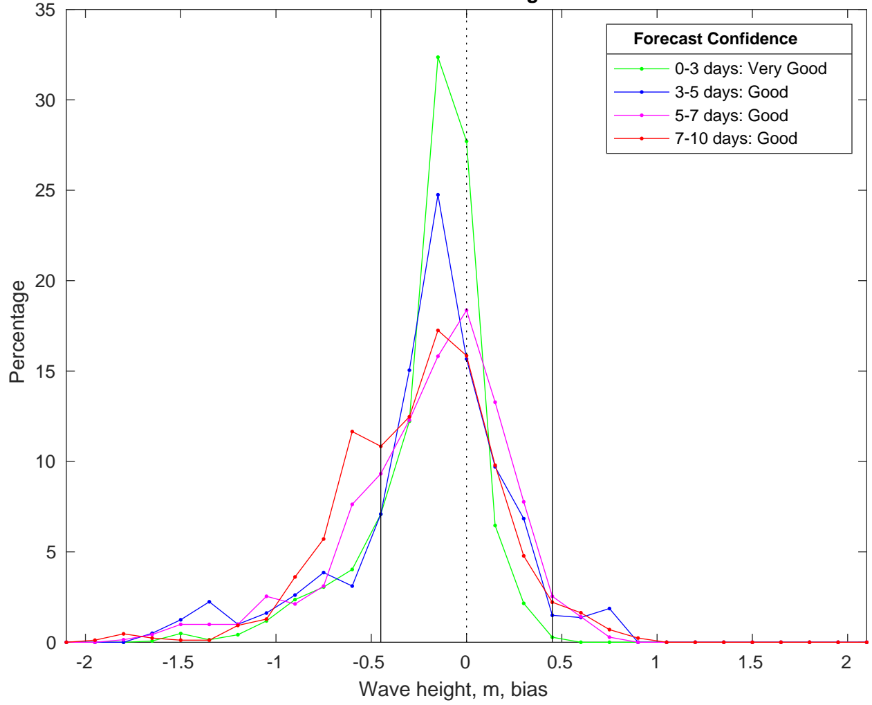
NDBC 42020 vs CMEMS Waves Bias Histogram: 08-Mar-2025
