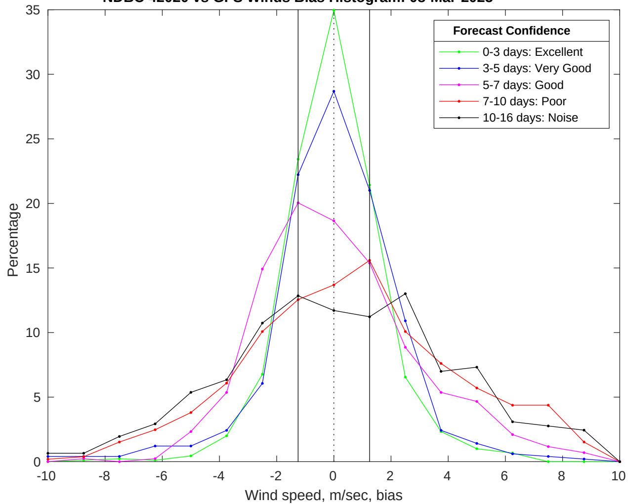
NDBC 42020 vs GFS Winds Bias Histogram: 08-Mar-2025
