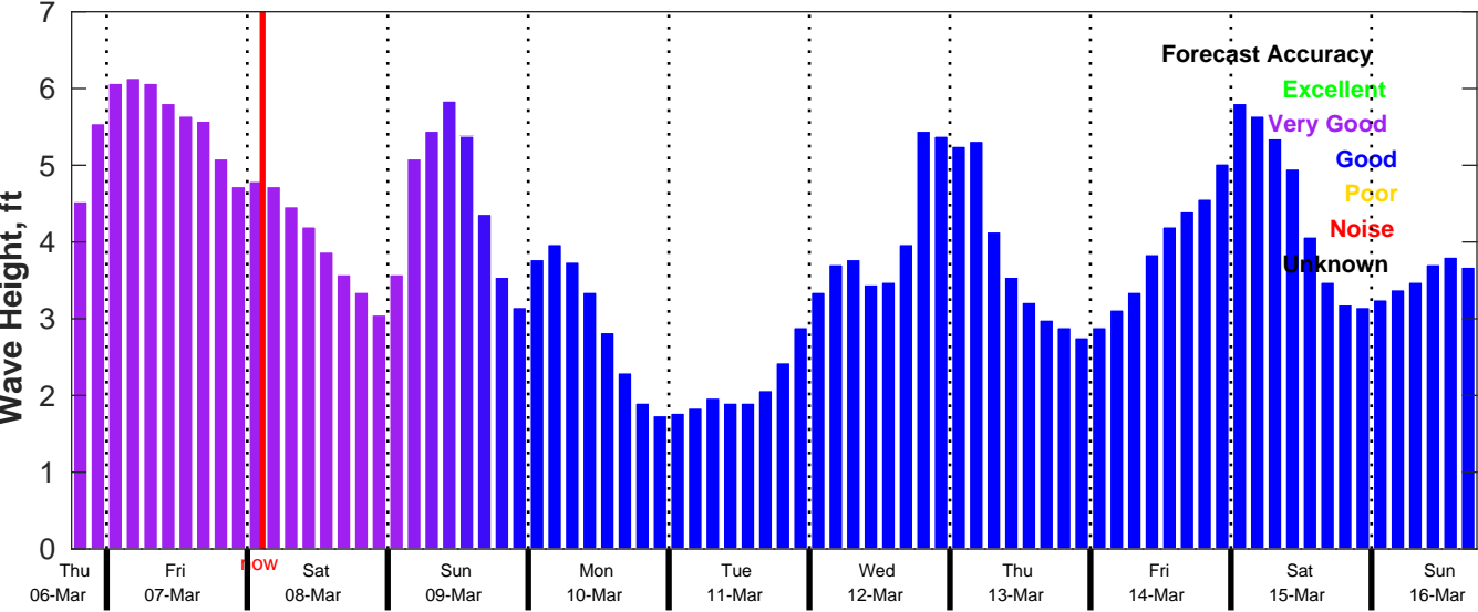
CMEMS Wave Forecast for NDBC 42020 from 06-Mar-2025 18:00:00 to 16-Mar-2025 18:00:00
