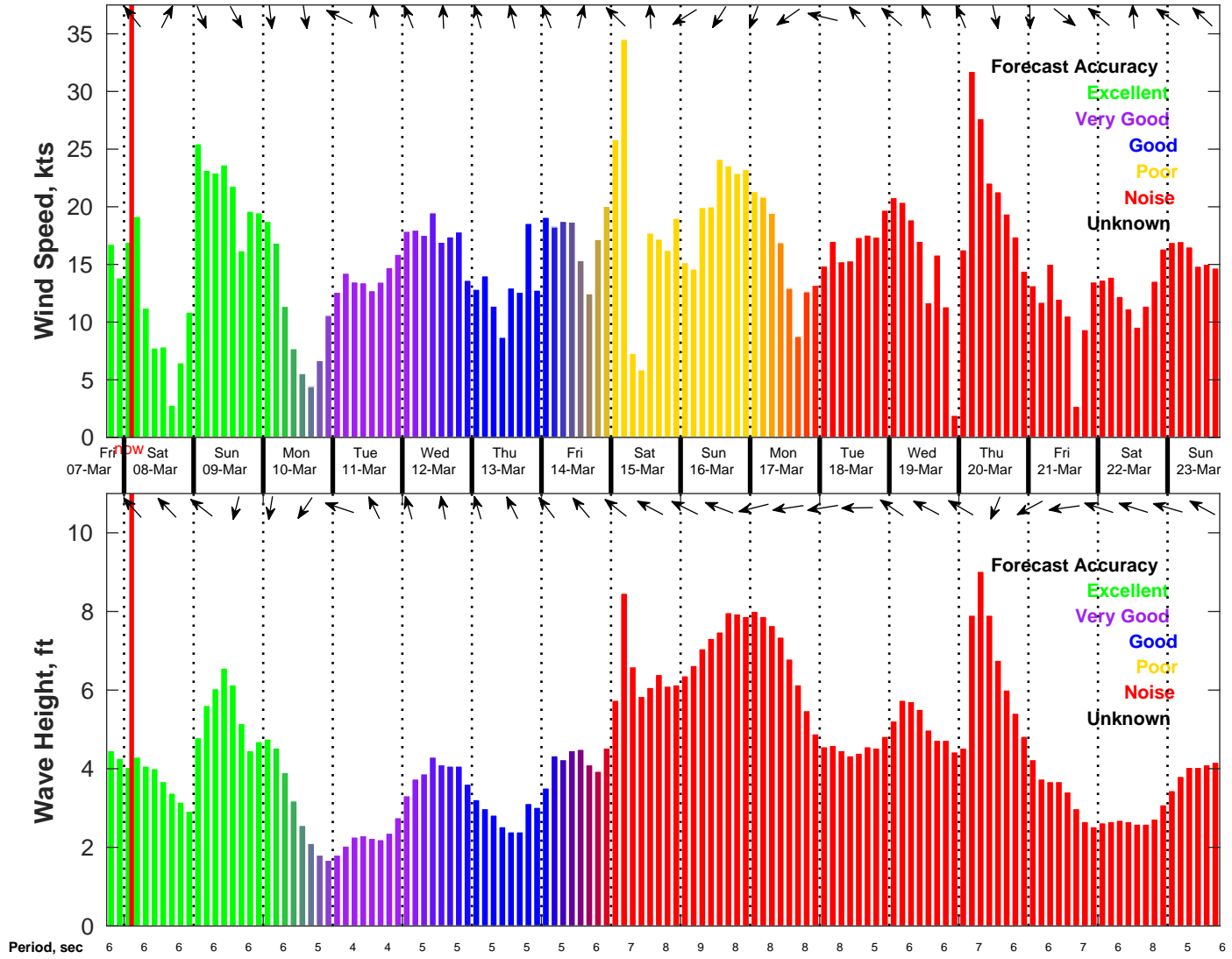
Wind & Wave Forecast for NDBC 42020 from 07-Mar-2025 18:00:00 to 23-Mar-2025 18:00:00
