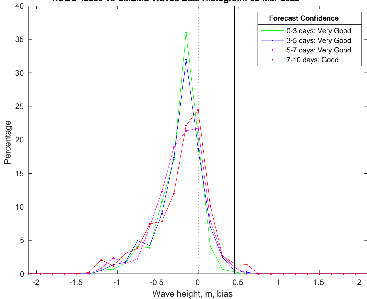
NDBC 42035 vs CMEMS Waves Bias Histogram: 08-Mar-2025
