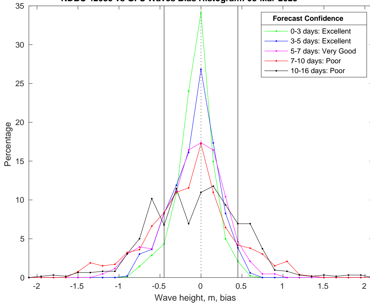
NDBC 42035 vs GFS Waves Bias Histogram: 08-Mar-2025
