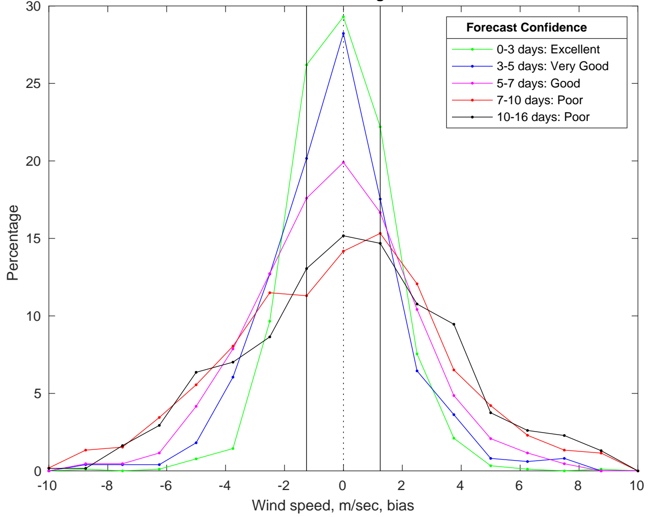
NDBC 42035 vs GFS Winds Bias Histogram: 08-Mar-2025
