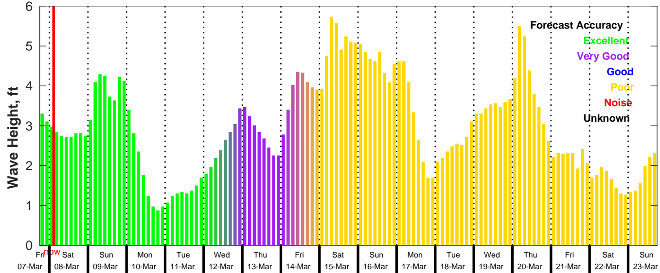
GFS Wave Forecast for NDBC 42035 from 07-Mar-2025 18:00:00 to 23-Mar-2025 18:00:00
