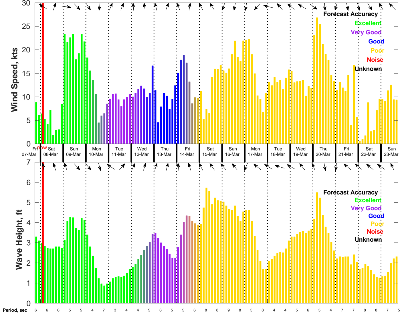
Wind & Wave Forecast for NDBC 42035 from 07-Mar-2025 18:00:00 to 23-Mar-2025 18:00:00
