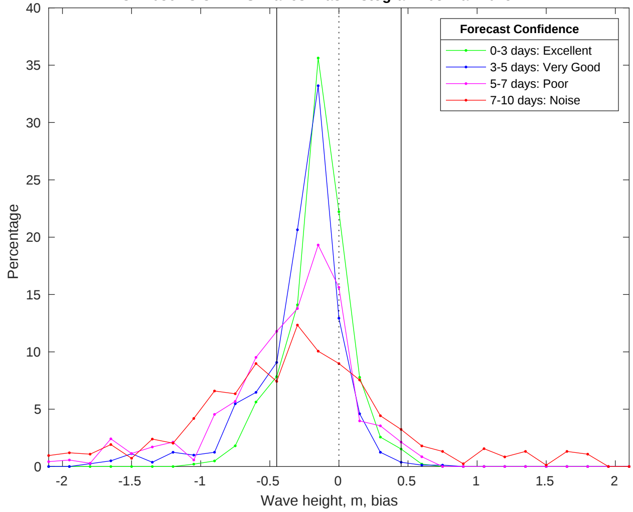
NDBC 42036 vs CMEMS Waves Bias Histogram: 08-Mar-2025
