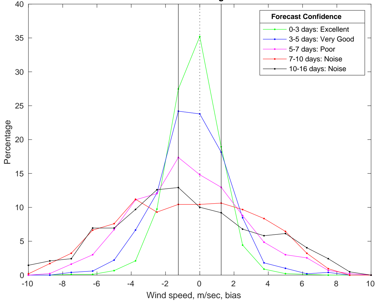
NDBC 42036 vs GFS Winds Bias Histogram: 08-Mar-2025
