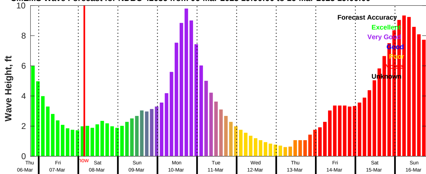
CMEMS Wave Forecast for NDBC 42036 from 06-Mar-2025 19:00:00 to 16-Mar-2025 19:00:00
