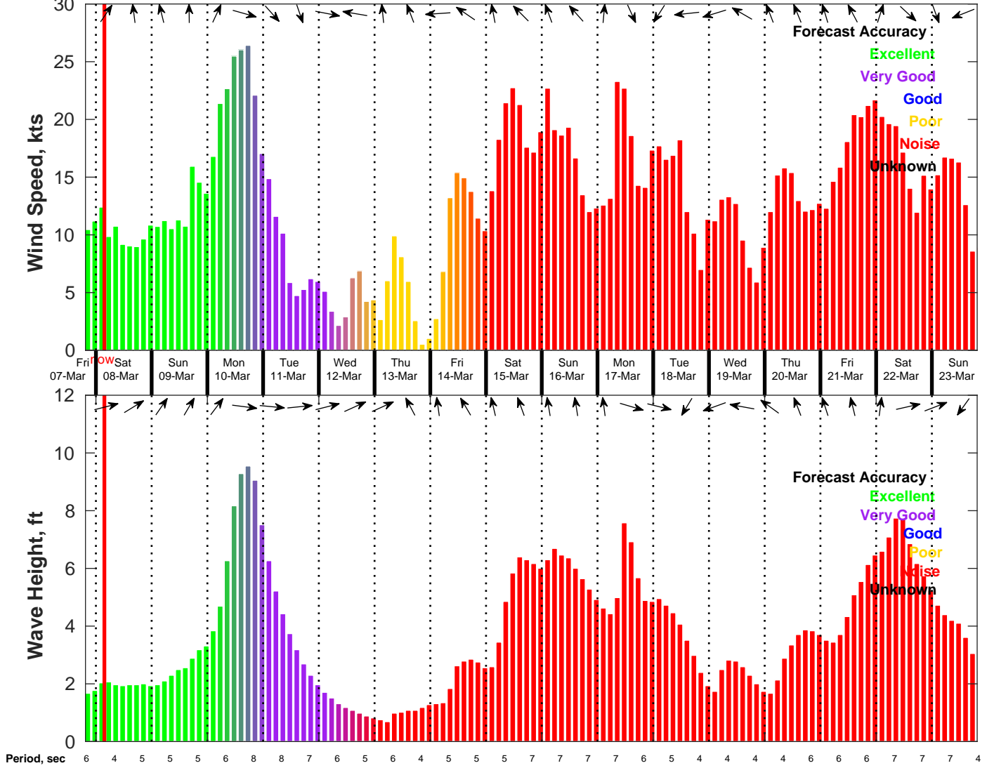
Wind & Wave Forecast for NDBC 42036 from 07-Mar-2025 19:00:00 to 23-Mar-2025 19:00:00
