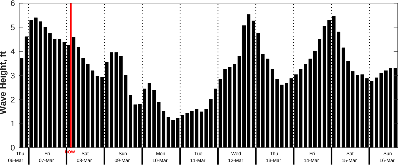
CMEMS Wave Forecast for NDBC 42092 from 06-Mar-2025 18:00:00 to 16-Mar-2025 18:00:00
