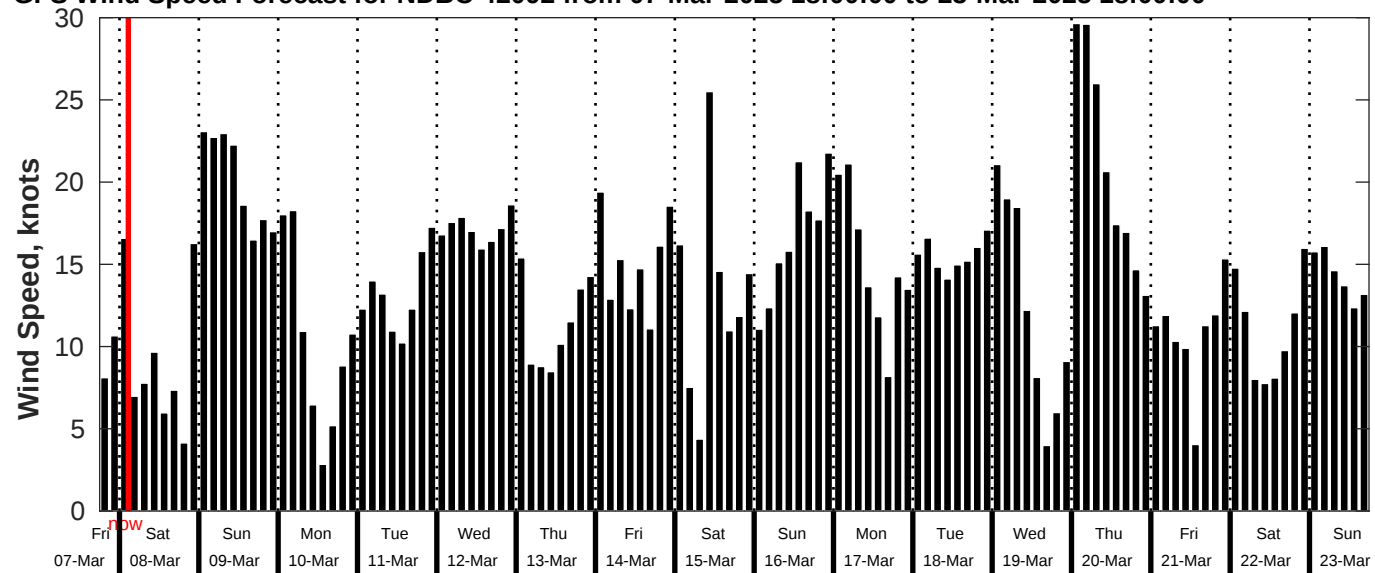
GFS Wind Speed Forecast for NDBC 42092 from 07-Mar-2025 18:00:00 to 23-Mar-2025 18:00:00
