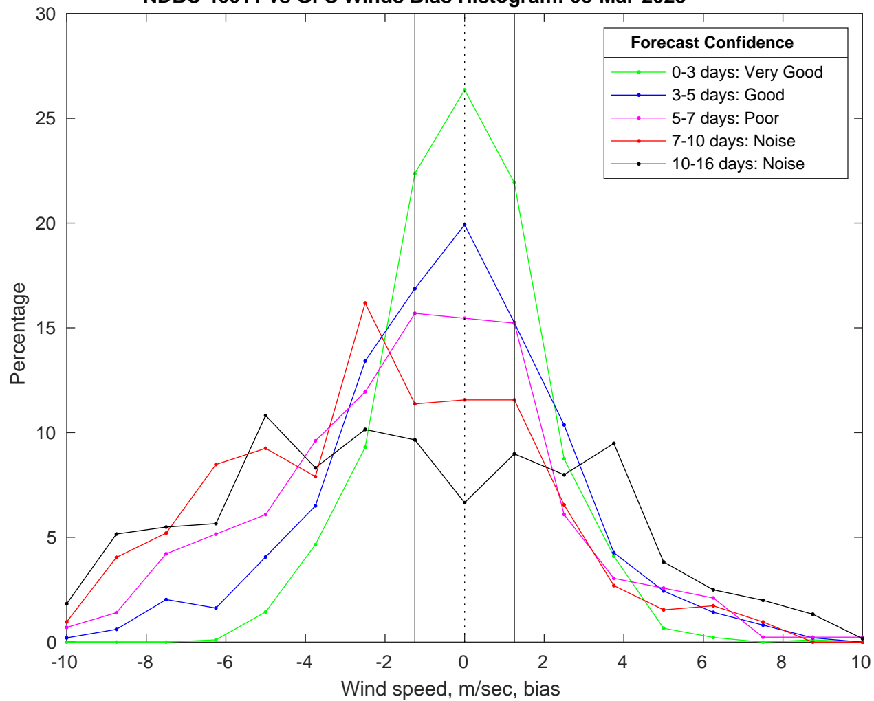
NDBC 46011 vs GFS Winds Bias Histogram: 08-Mar-2025
