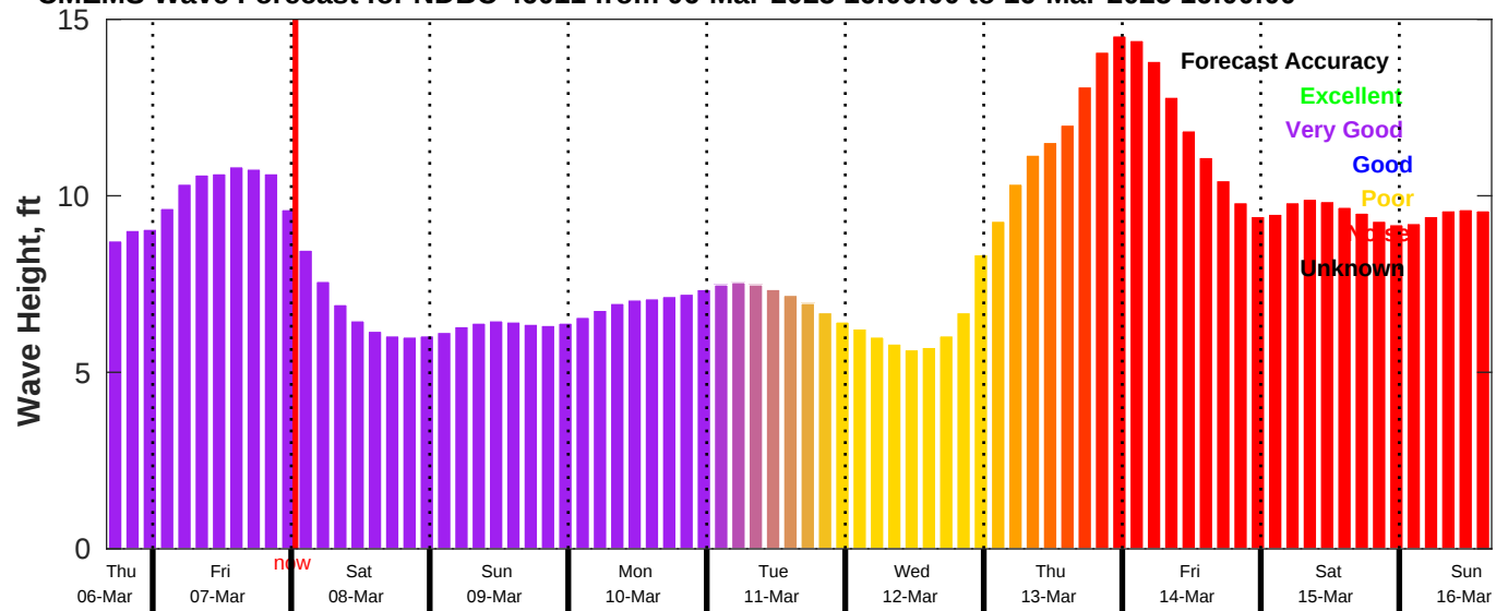
CMEMS Wave Forecast for NDBC 46011 from 06-Mar-2025 16:00:00 to 16-Mar-2025 16:00:00
