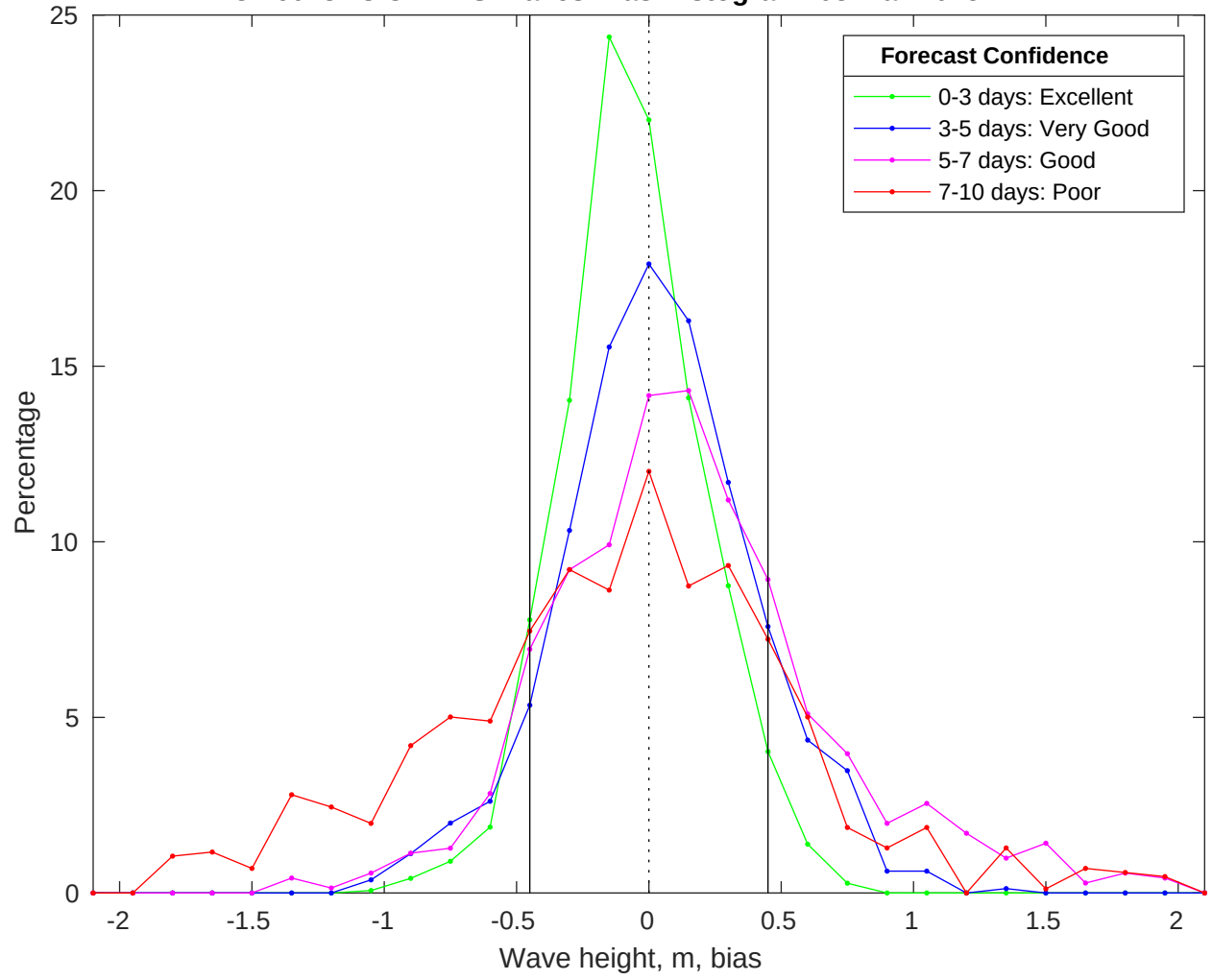
NDBC 46028 vs CMEMS Waves Bias Histogram: 08-Mar-2025
