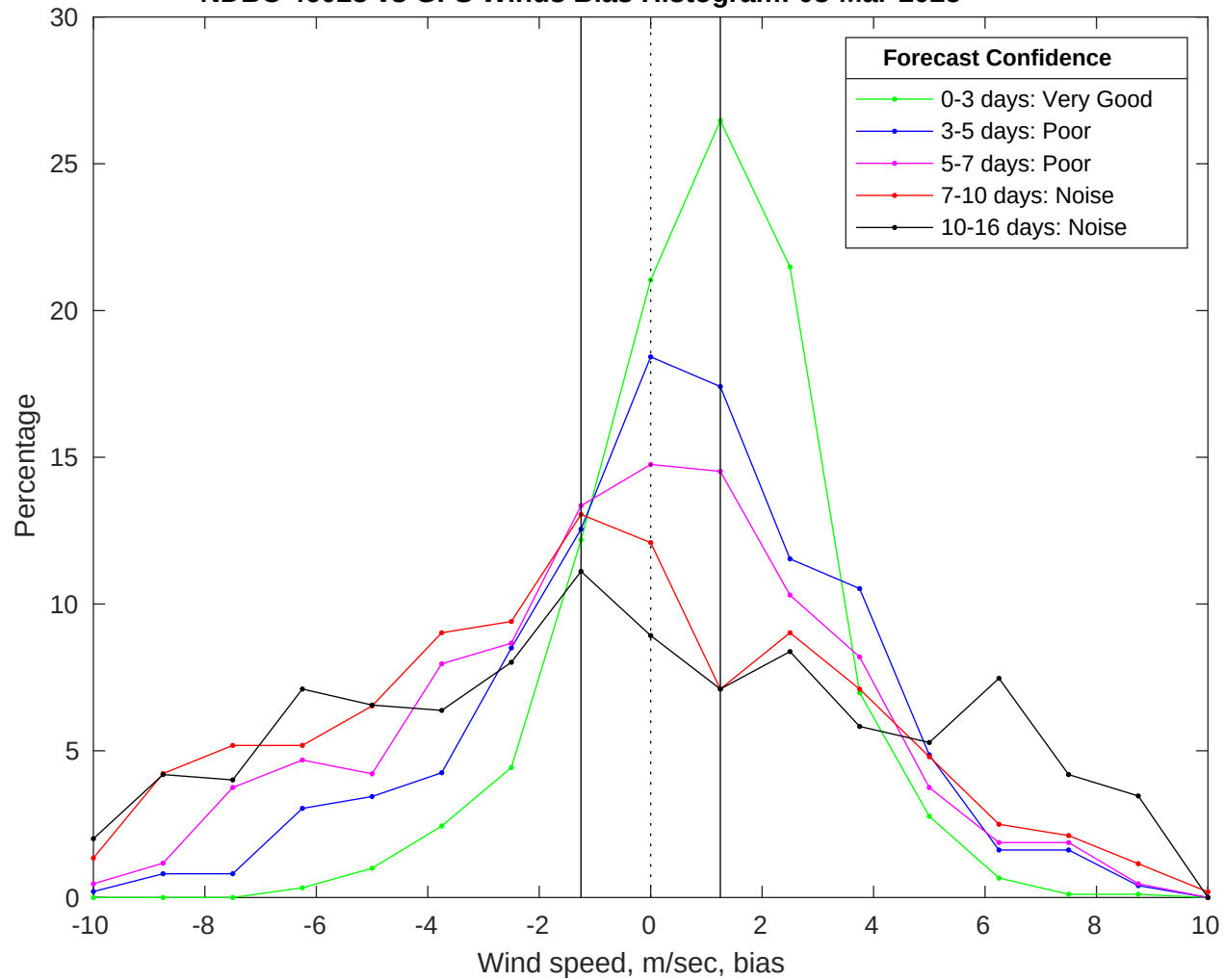
NDBC 46028 vs GFS Winds Bias Histogram: 08-Mar-2025
