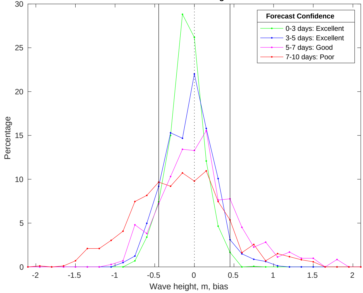
NDBC 46054 vs CMEMS Waves Bias Histogram: 08-Mar-2025
