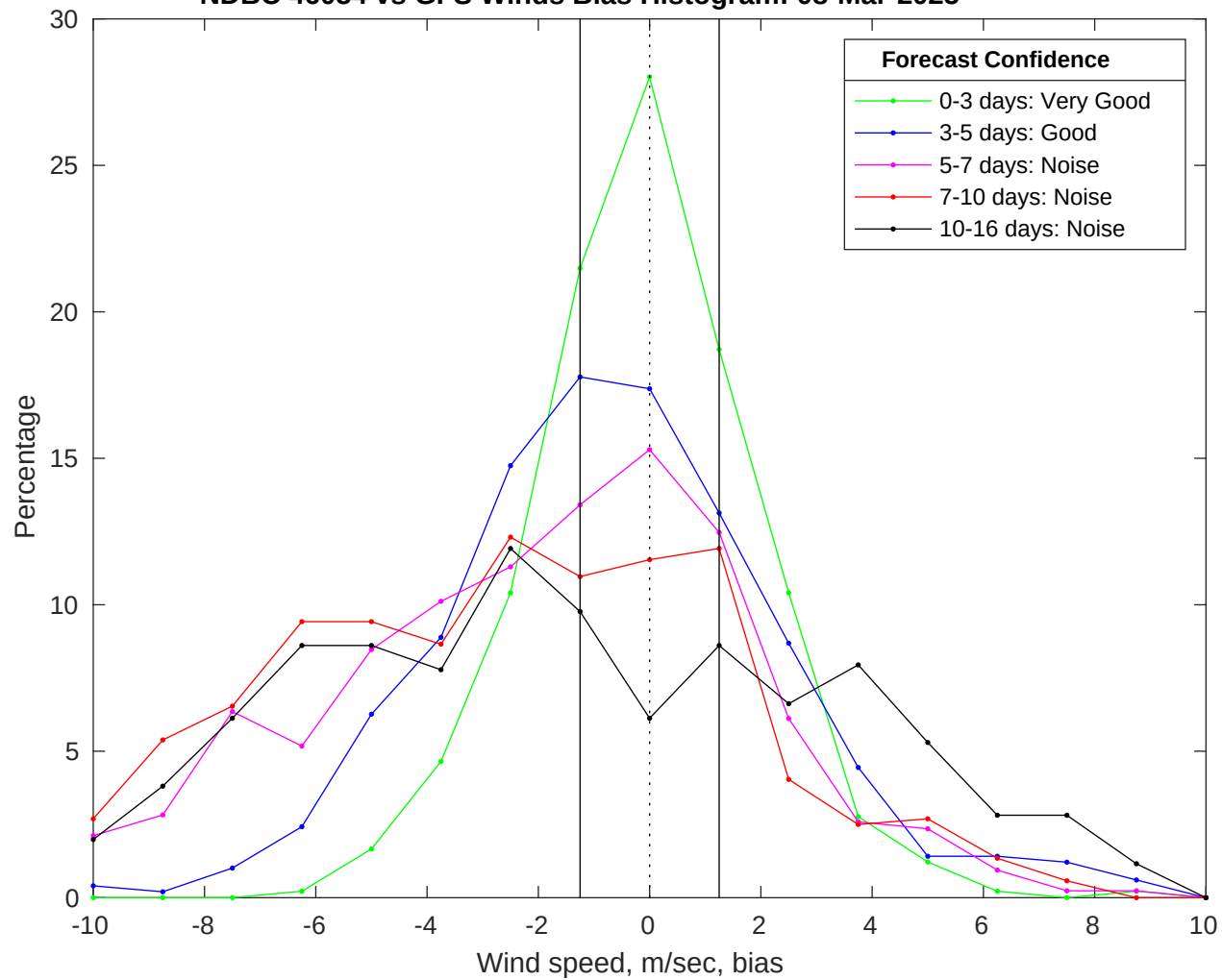
NDBC 46054 vs GFS Winds Bias Histogram: 08-Mar-2025
