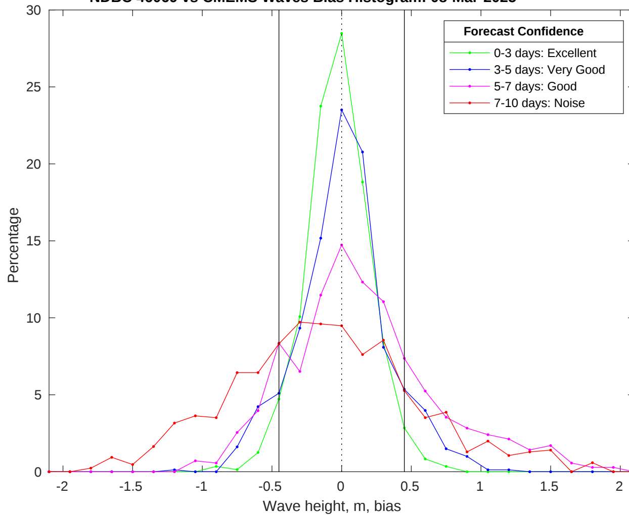
NDBC 46069 vs CMEMS Waves Bias Histogram: 08-Mar-2025
