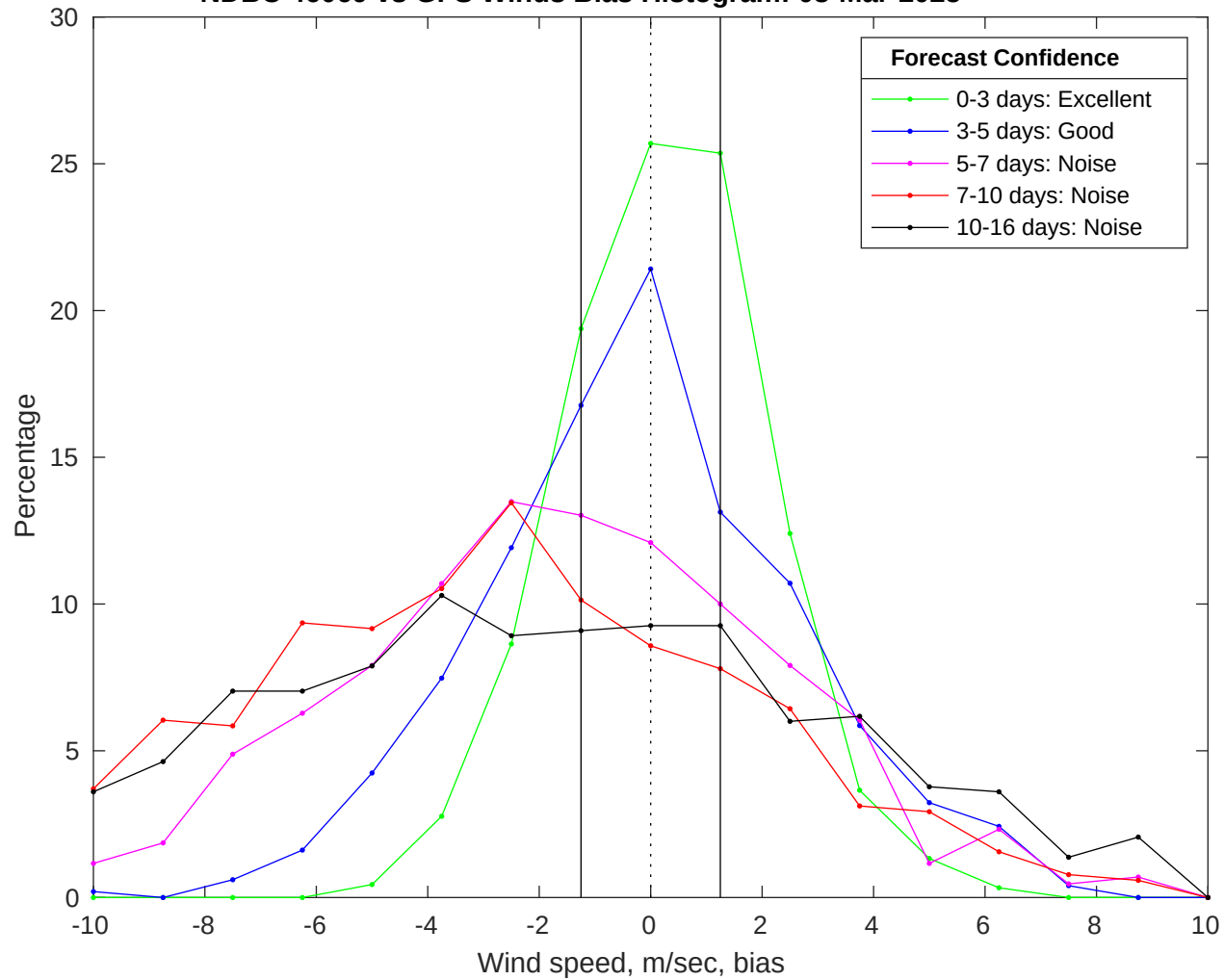
NDBC 46069 vs GFS Winds Bias Histogram: 08-Mar-2025
