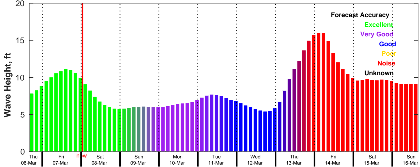
CMEMS Wave Forecast for NDBC 46069 from 06-Mar-2025 16:00:00 to 16-Mar-2025 16:00:00
