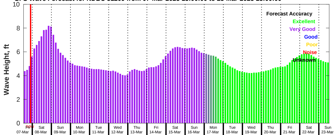
GFS Wave Forecast for NDBC 51209 from 07-Mar-2025 13:00:00 to 23-Mar-2025 13:00:00
