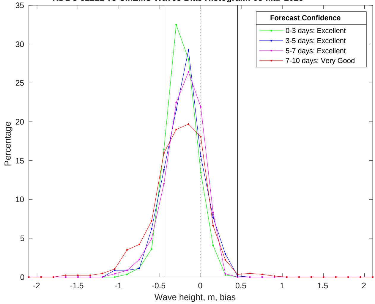
NDBC 52211 vs CMEMS Waves Bias Histogram: 08-Mar-2025
