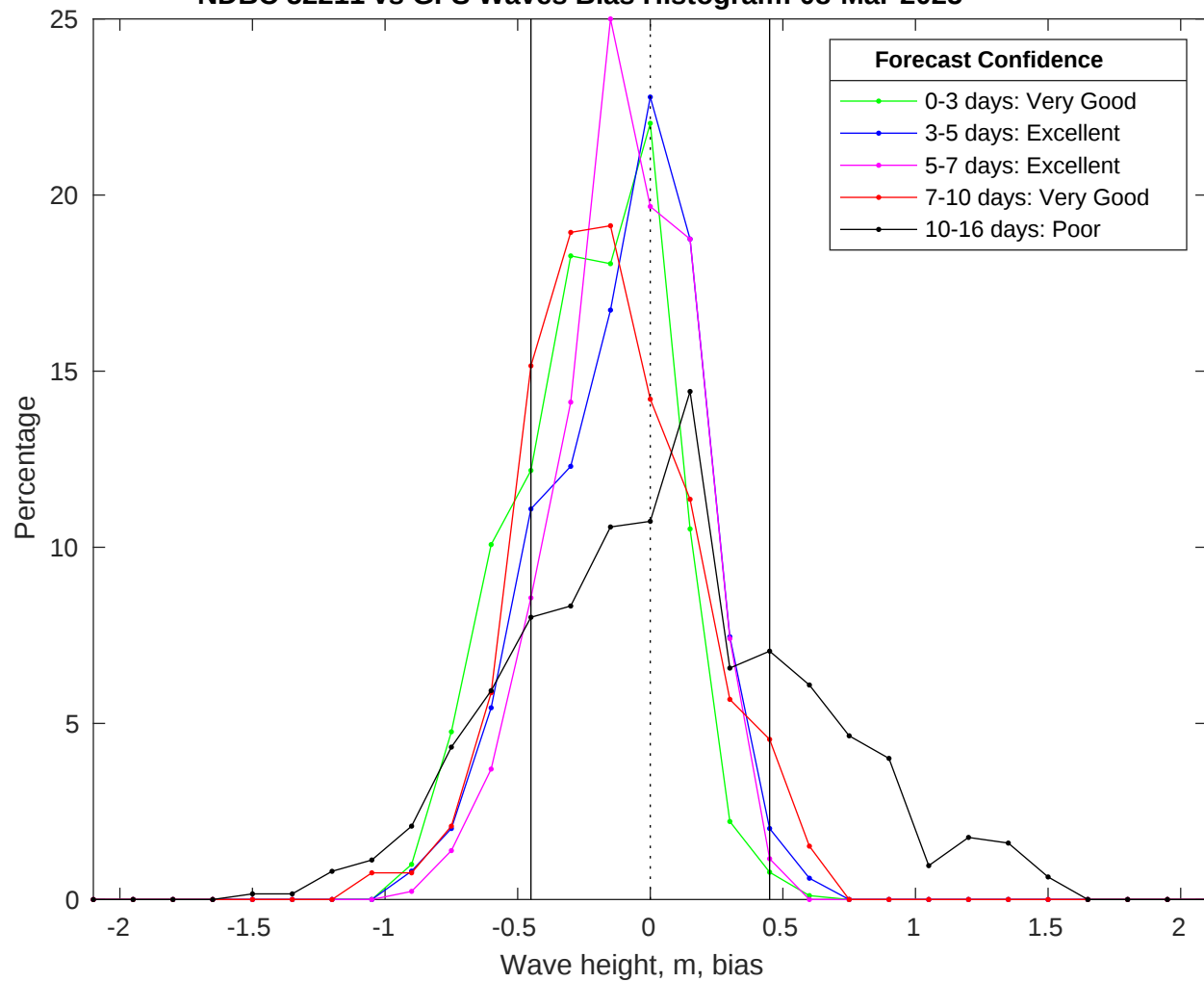
NDBC 52211 vs GFS Waves Bias Histogram: 08-Mar-2025
