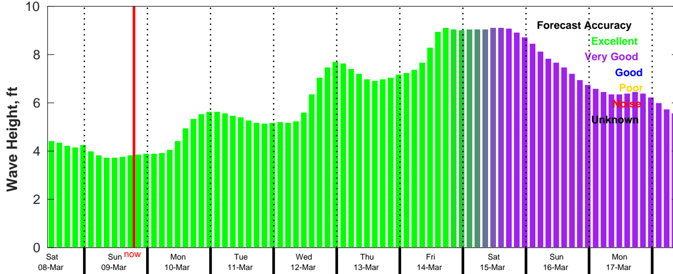
CMEMS Wave Forecast for NDBC 52211 from 07-Mar-2025 10:00:00 to 17-Mar-2025 10:00:00
