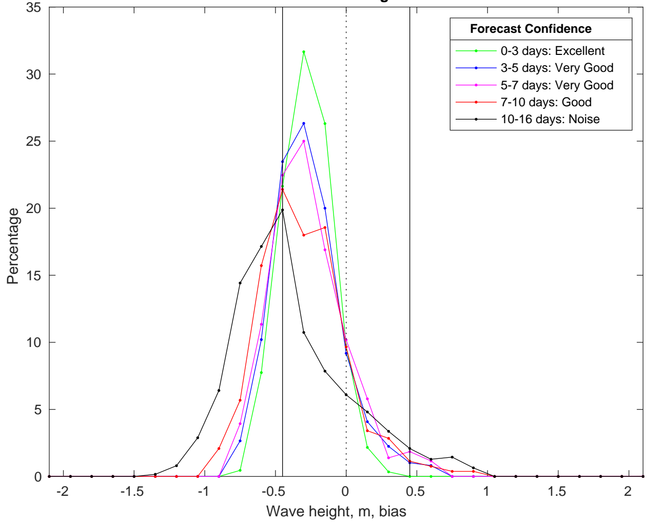
NDBC 52212 vs GFS Waves Bias Histogram: 08-Mar-2025
