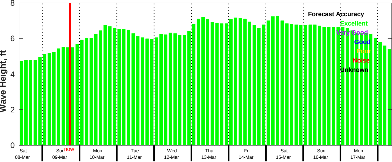
CMEMS Wave Forecast for NDBC 52212 from 07-Mar-2025 09:00:00 to 17-Mar-2025 09:00:00
