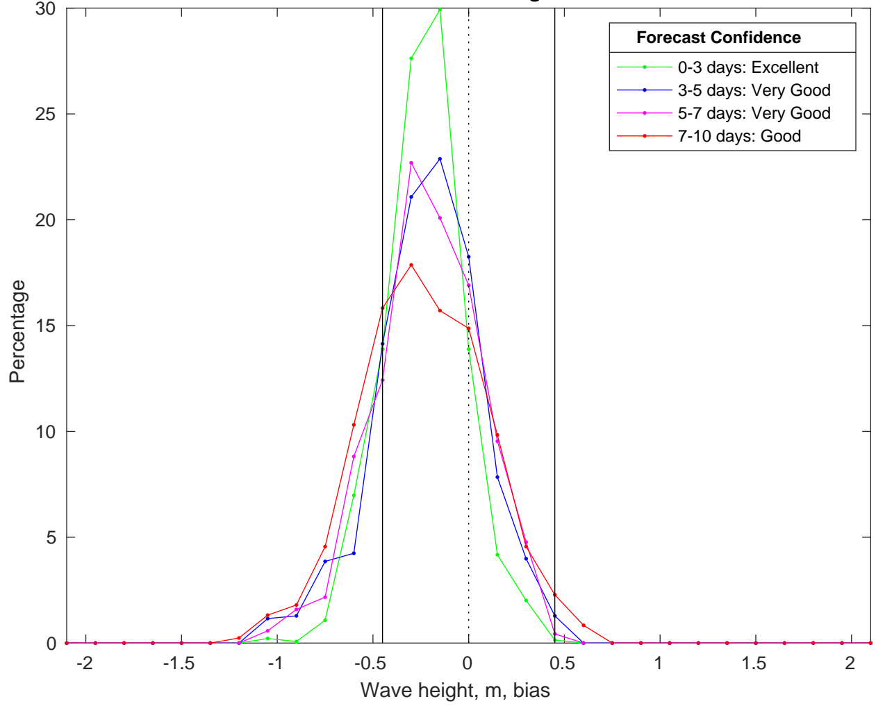
NDBC 52213 vs CMEMS Waves Bias Histogram: 08-Mar-2025
