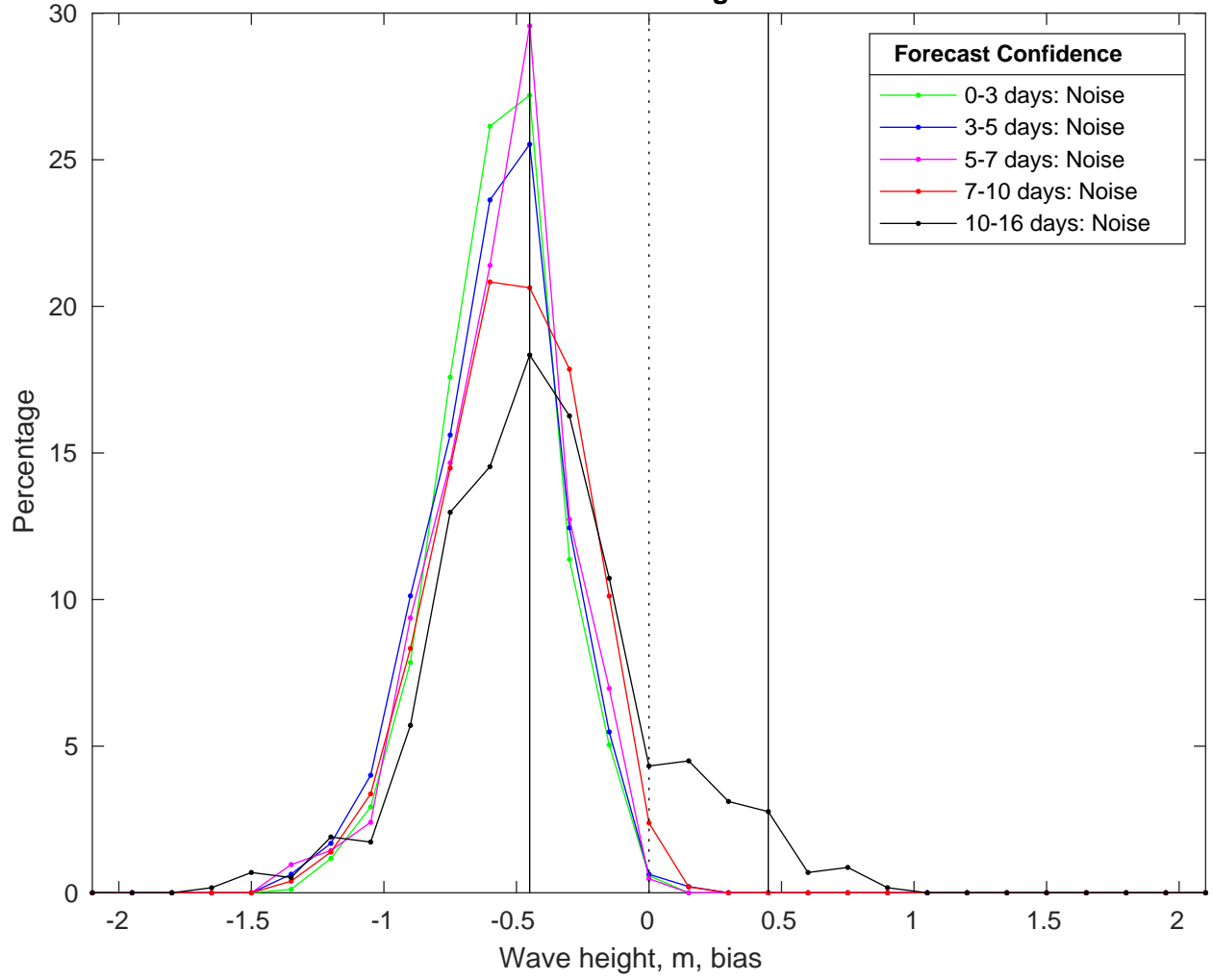
NDBC 52213 vs GFS Waves Bias Histogram: 08-Mar-2025
