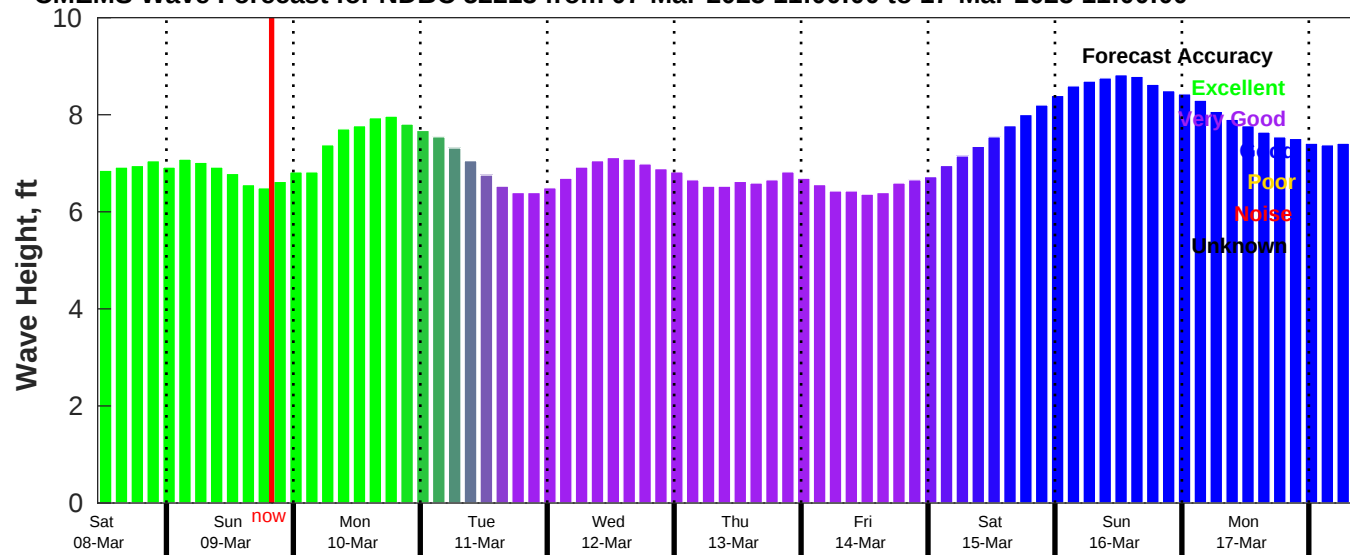
CMEMS Wave Forecast for NDBC 52213 from 07-Mar-2025 11:00:00 to 17-Mar-2025 11:00:00
