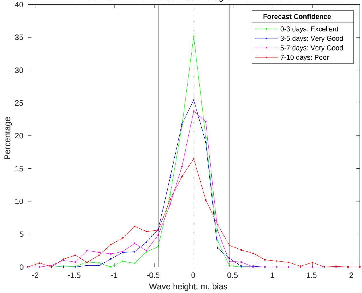
NDBC 41004 vs CMEMS Waves Bias Histogram: 09-Mar-2025
