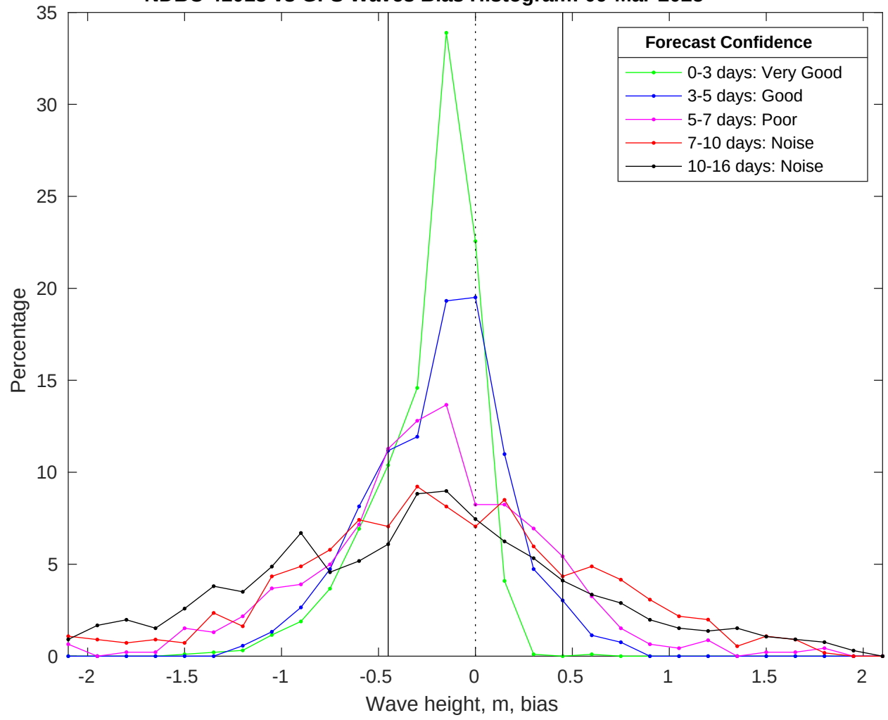
NDBC 41013 vs GFS Waves Bias Histogram: 09-Mar-2025
