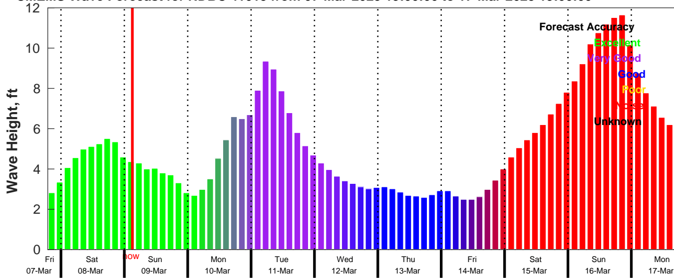
CEEMS Wave Forecast for NDBC 41013 from 07-Mar-2025 19:00:00 to 17-Mar-2025 19:00:00
