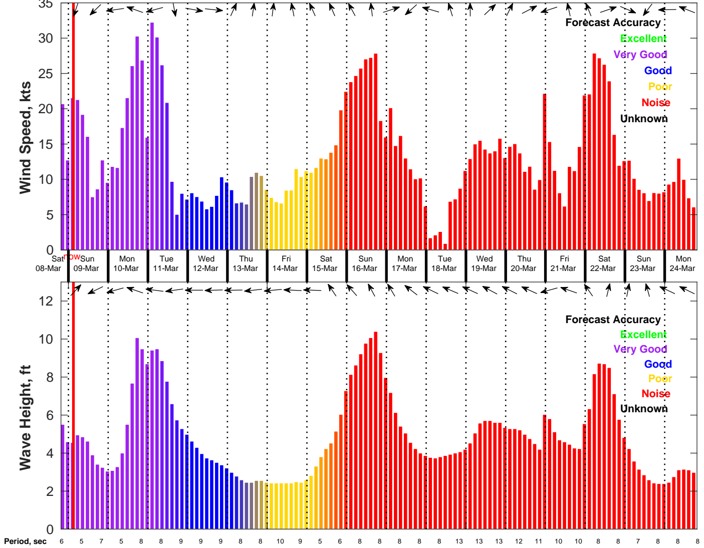
Wind & Wave Forecast for NDBC 41013 from 08-Mar-2025 19:00:00 to 24-Mar-2025 19:00:00
