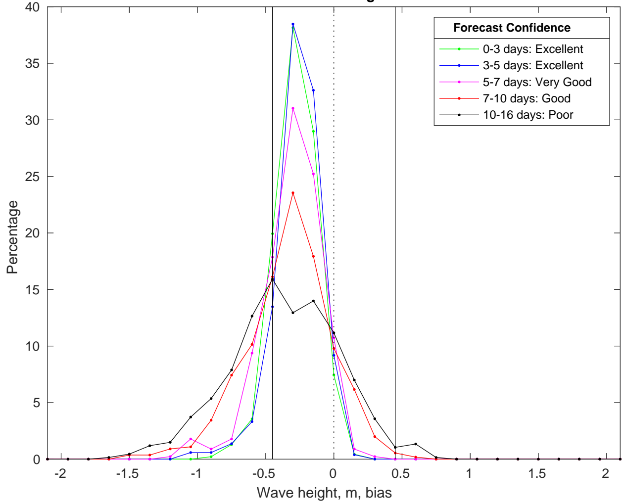
NDBC 41040 vs GFS Waves Bias Histogram: 09-Mar-2025
