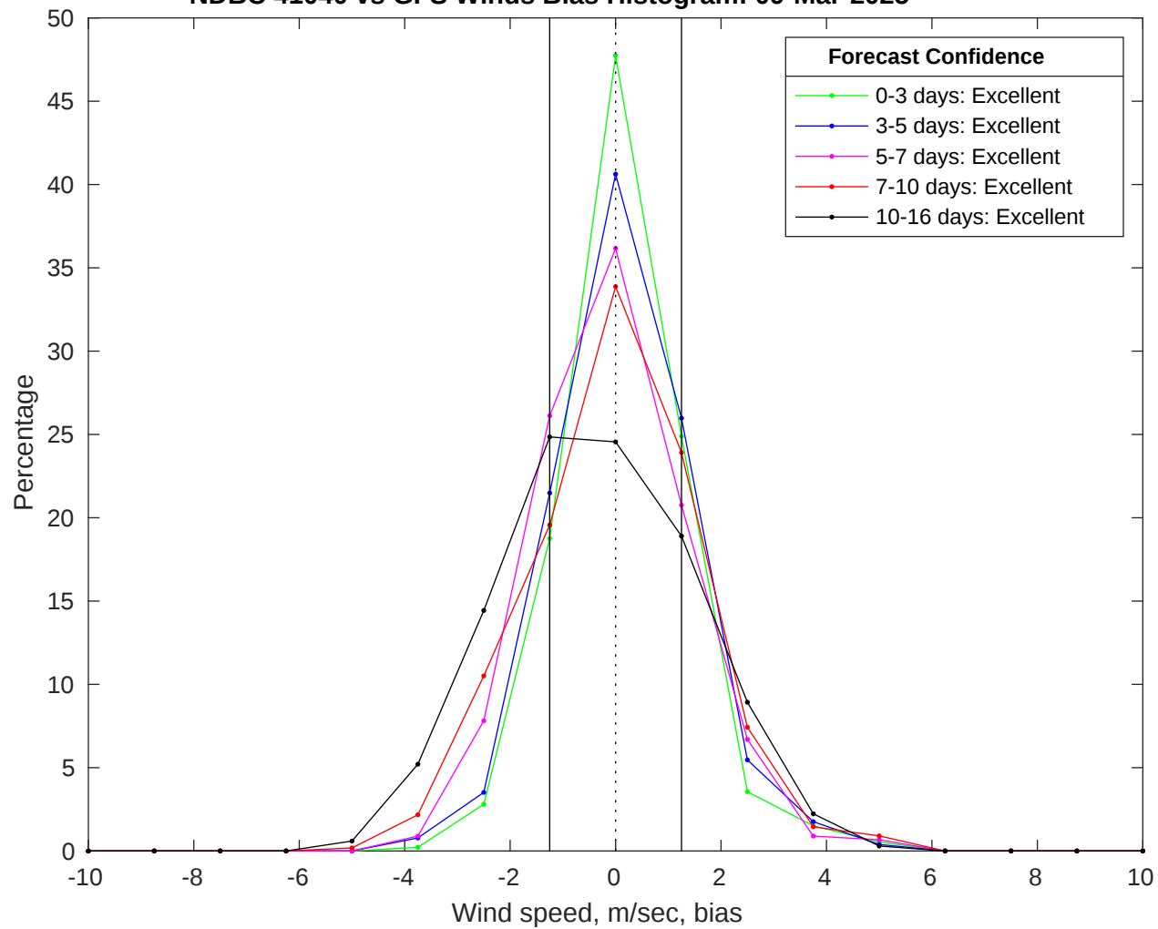
NDBC 41040 vs GFS Winds Bias Histogram: 09-Mar-2025
